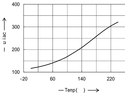
\mu iac vs. Temperature \mu iac温度特性
