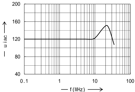
\mu iac vs. Frequency \mu iac周波数特性
