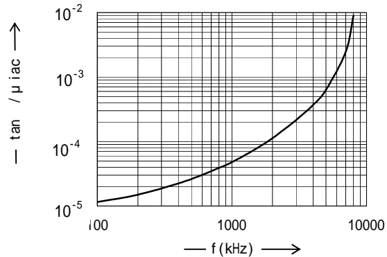
\tan \delta / \mu_{iac} vs. Frequency \tan \delta / \mu_{iac} 周波数特性
