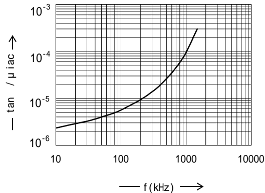
\tan / \mu_{iac} vs. Frequency \tan / \mu_{iac} 周波数特性
