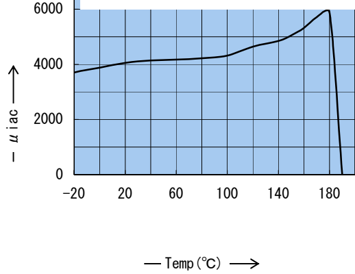
\mu_{iac} vs. Temperature \mu_{iac} 温度特性
