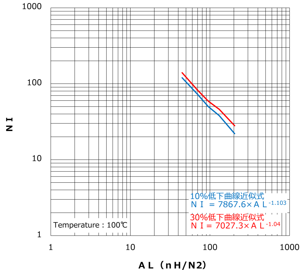
NI v s AL-value (typ)
