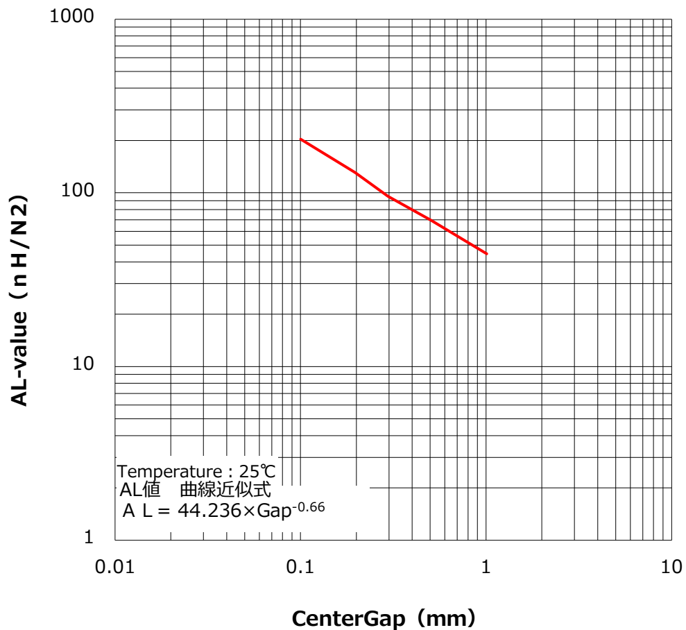
AL-value v s CenterGap (typ)
