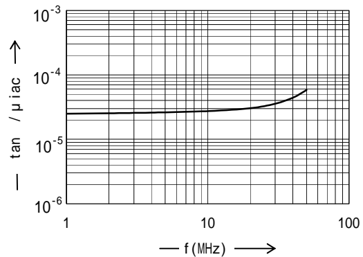
\tan / \mu iac vs. Frequency \tan / \mu iac周波数特性
