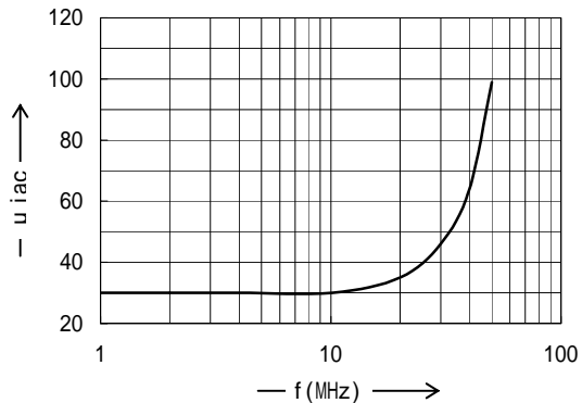
\mu iac vs. Frequency \mu iac周波数特性
