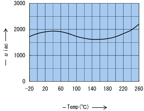
\mu_{iac} vs. Temperature \mu_{iac} 温度特性
