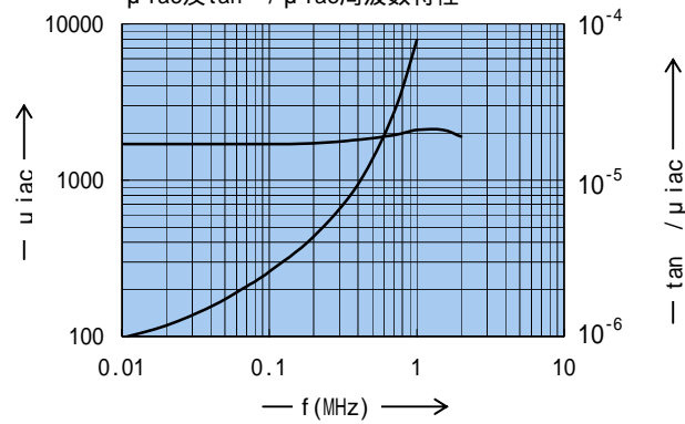
\mu_{iac} and \tan \delta / \mu_{iac} vs. Frequency \mu_{iac} 及 \tan \delta / \mu_{iac} 周波数特性
