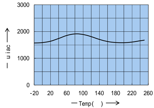
\mu_{iac} vs. Temperature \mu_{iac} 温度特性
