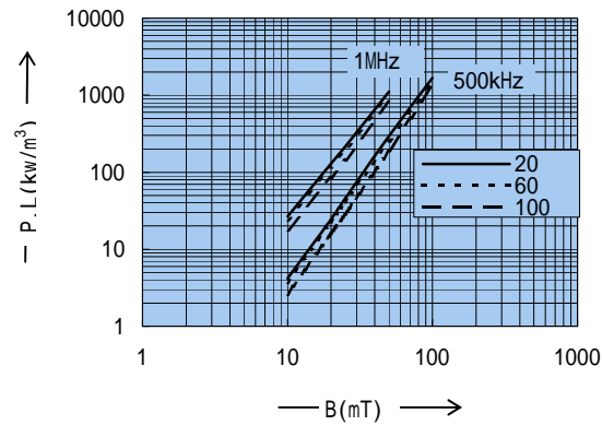
Power loss vs. Flux density P_L vs. B vs. 磁束密度
