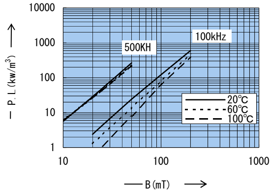
Power loss vs. Flux density P_w - B vs. 磁束密度
