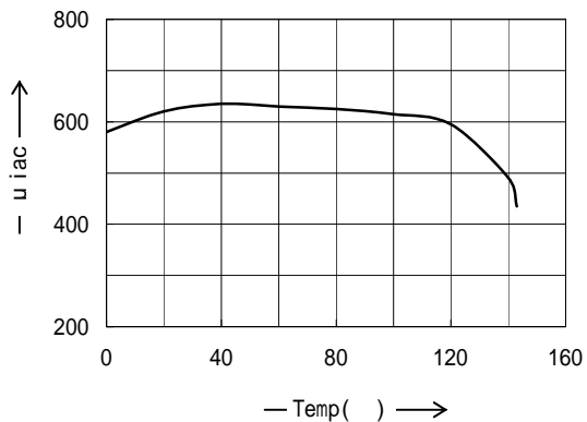
\mu iac vs. Temperature \mu iac温度特性
